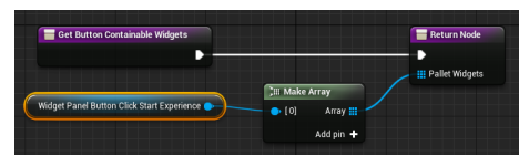
Figure 61. Code Example: Get Buttons Function.
